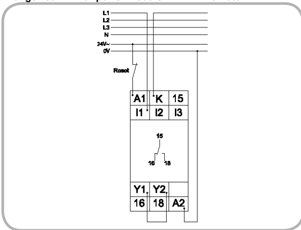
► Range 10A with power module 400V AC without latch
